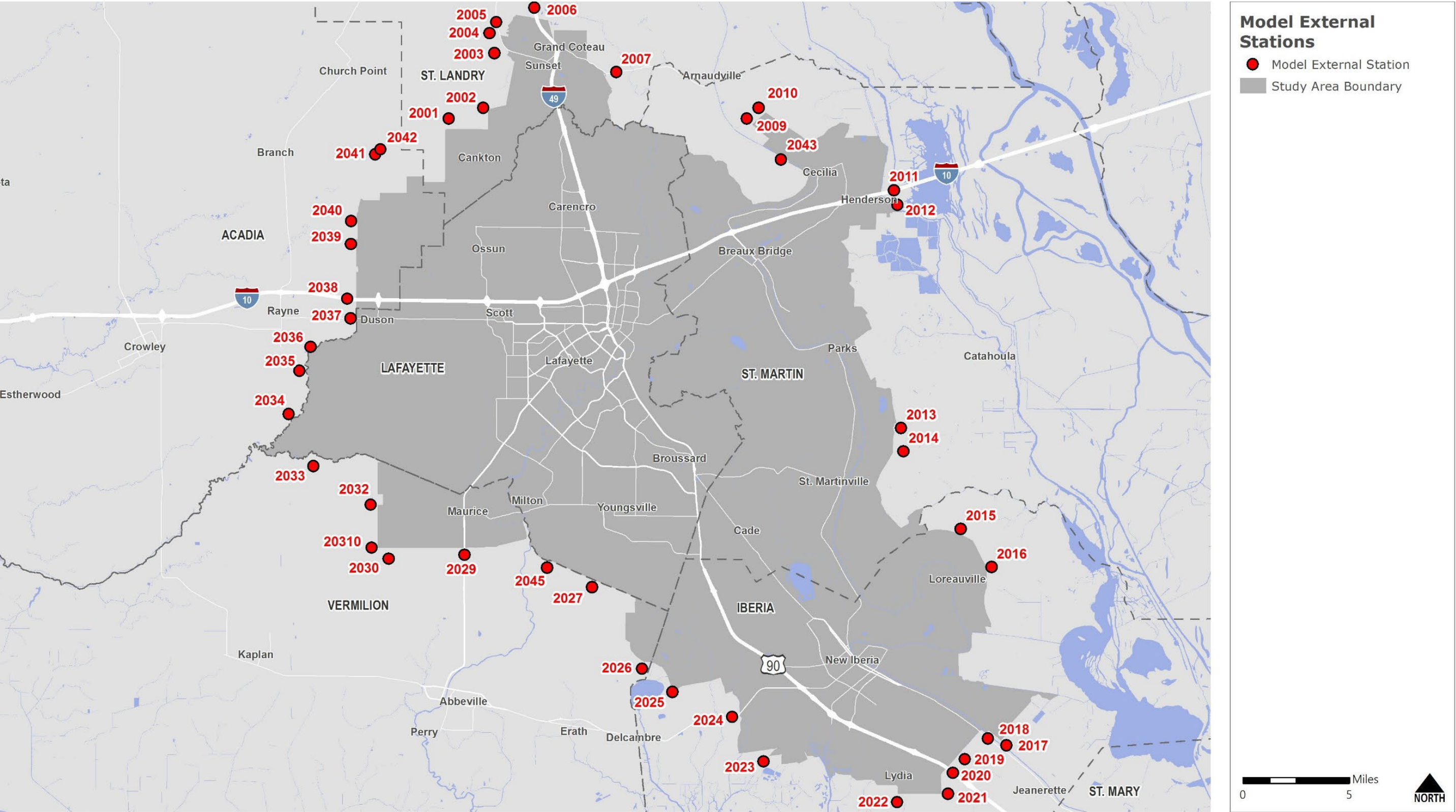
Figure 4.1: Model External Stations
