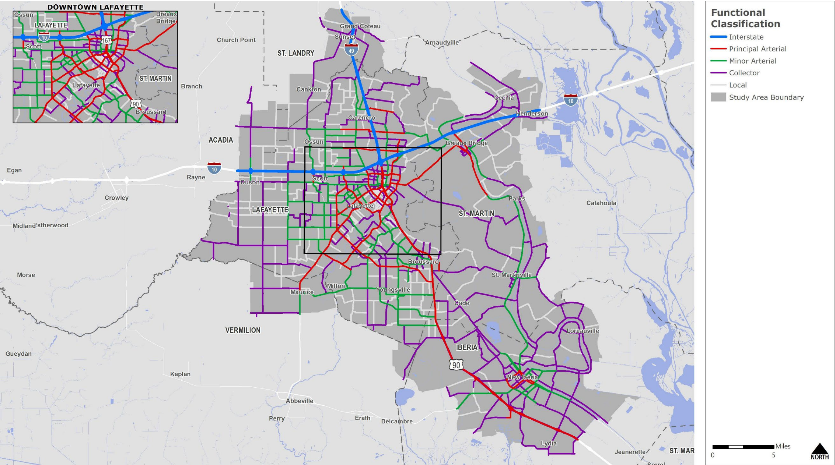
Figure 3.1: Roadway Network and Functional Classification, Base Year
